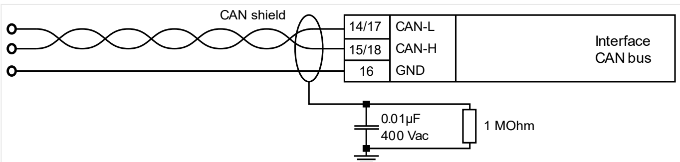
Fig. 13: Shielding CAN bus - grounded (replacement of IKD1M)
