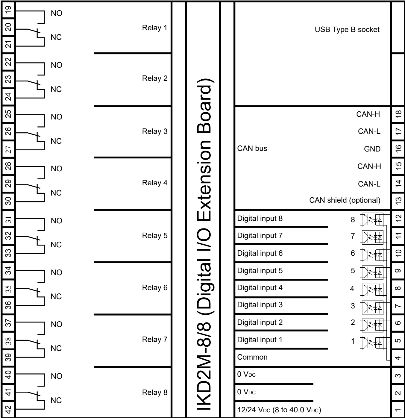
Fig. 5: Wiring Diagram
