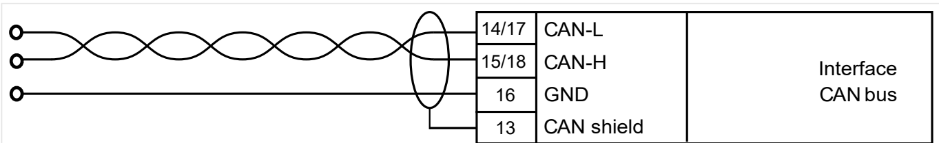
Fig. 12: Shielding CAN bus - connected to terminal
